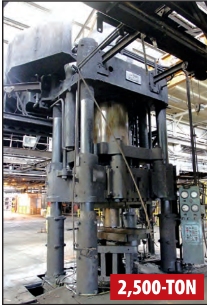
WATSON STILLMAN 4-POST HYDRAULIC FORGING PRESS
