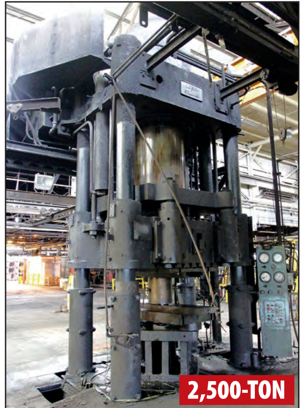
WATSON STILLMAN 4-POST HYDRAULIC FORGING PRESS
